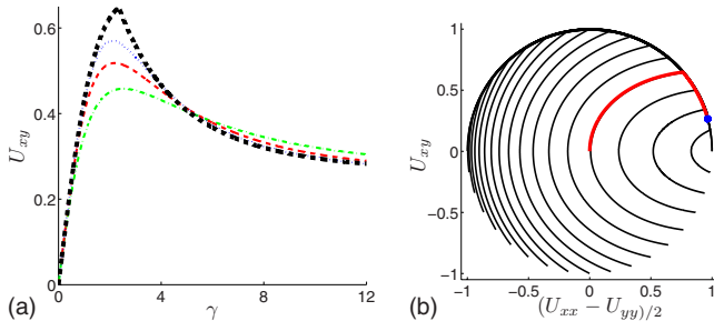
FIG. 12. (Color online) Representations of the model for U_Y = 1 . (a) U_{xy} versus \gamma for the first step and different yield functions, as in Fig. 6(a). (b) Representation of the model for \dot{\gamma} > 0 in component spaces for n \rightarrow +\infty , as in Fig. 9(b).
