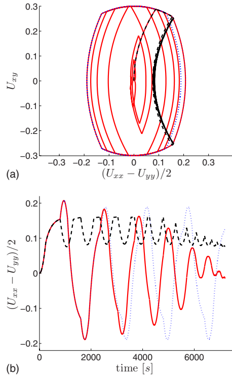
FIG. 11. (Color online) Shearing cycles to remove trapped stresses. Here U_i=0 for the first step and U_Y=0.3 , n \rightarrow +\infty . Between two steps: the direction of shearing is turned 90° clockwise (blue dots); the amplitude is decreased from \gamma=2 to 0 in 15 steps (black dashes); simultaneously, the direction of shear is turned and its amplitude is decreased (red solid line). (a) Component space. (b) (U_{xx}-U_{yy})/2 versus time ( |\dot{\gamma}|=2.5 \times 10^{-3} \text{ s}^{-1} ).
