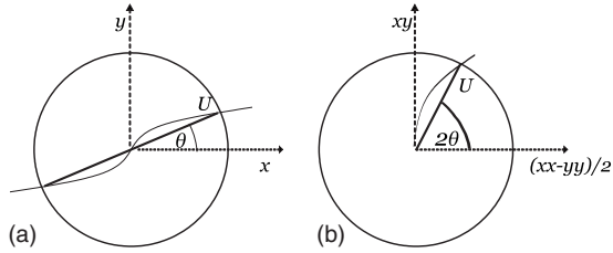
FIG. 4. Representation of the evolution of \bar{\mathbf{U}} . (a) Physical space: evolution of the point (U \cos \theta, U \sin \theta) ; for completeness we also plot the opposite (and strictly equivalent) point (-U \cos \theta, -U \sin \theta) . (b) Component space: trajectory of [(U_{xx} - U_{yy})/2, U_{xy}] , that is, (U \cos 2\theta, U \sin 2\theta) .
